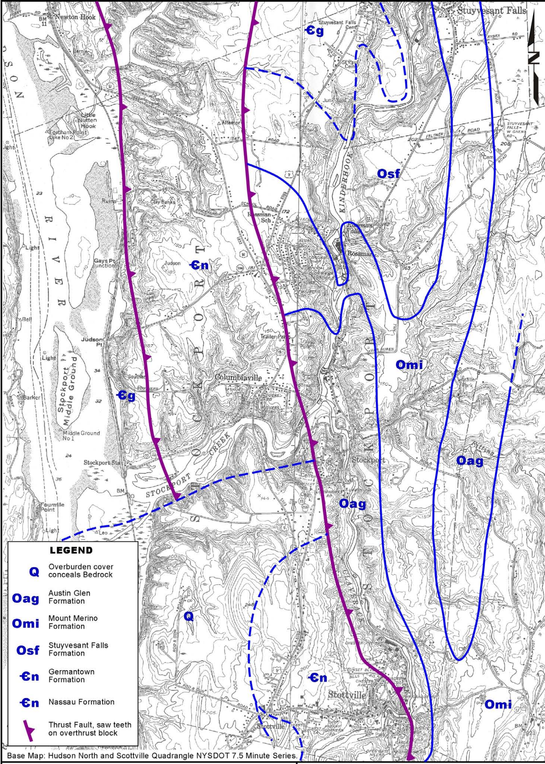
FIGURE 2 BEDROCK GEOLOGY MAP
